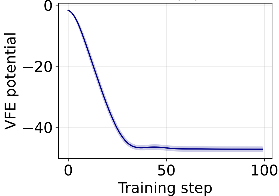
Neural VFE: \mathcal{F}(Z) descent
