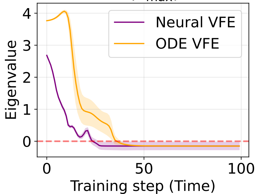
\text{Re}(\lambda_{\max})
