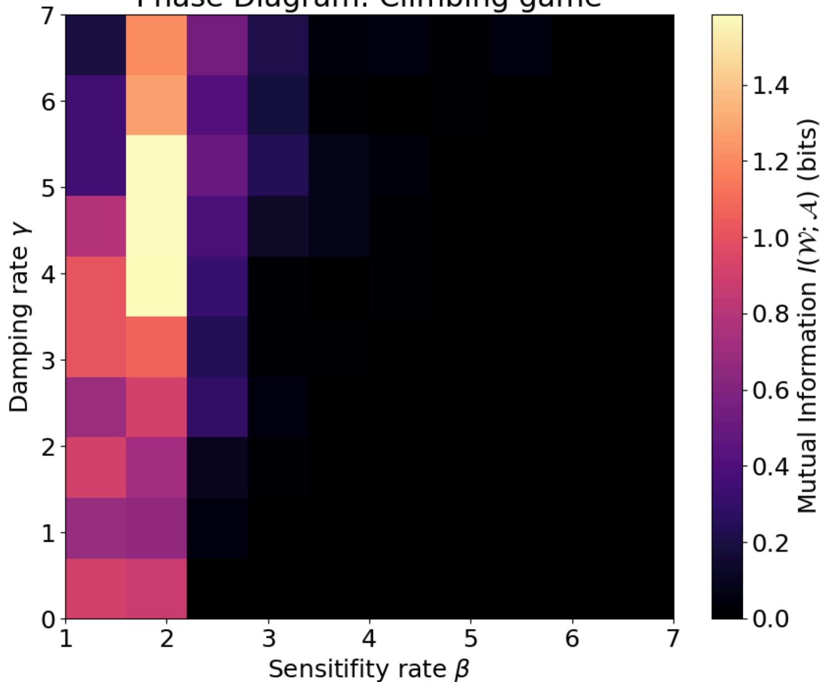
Phase Diagram: Climbing game
