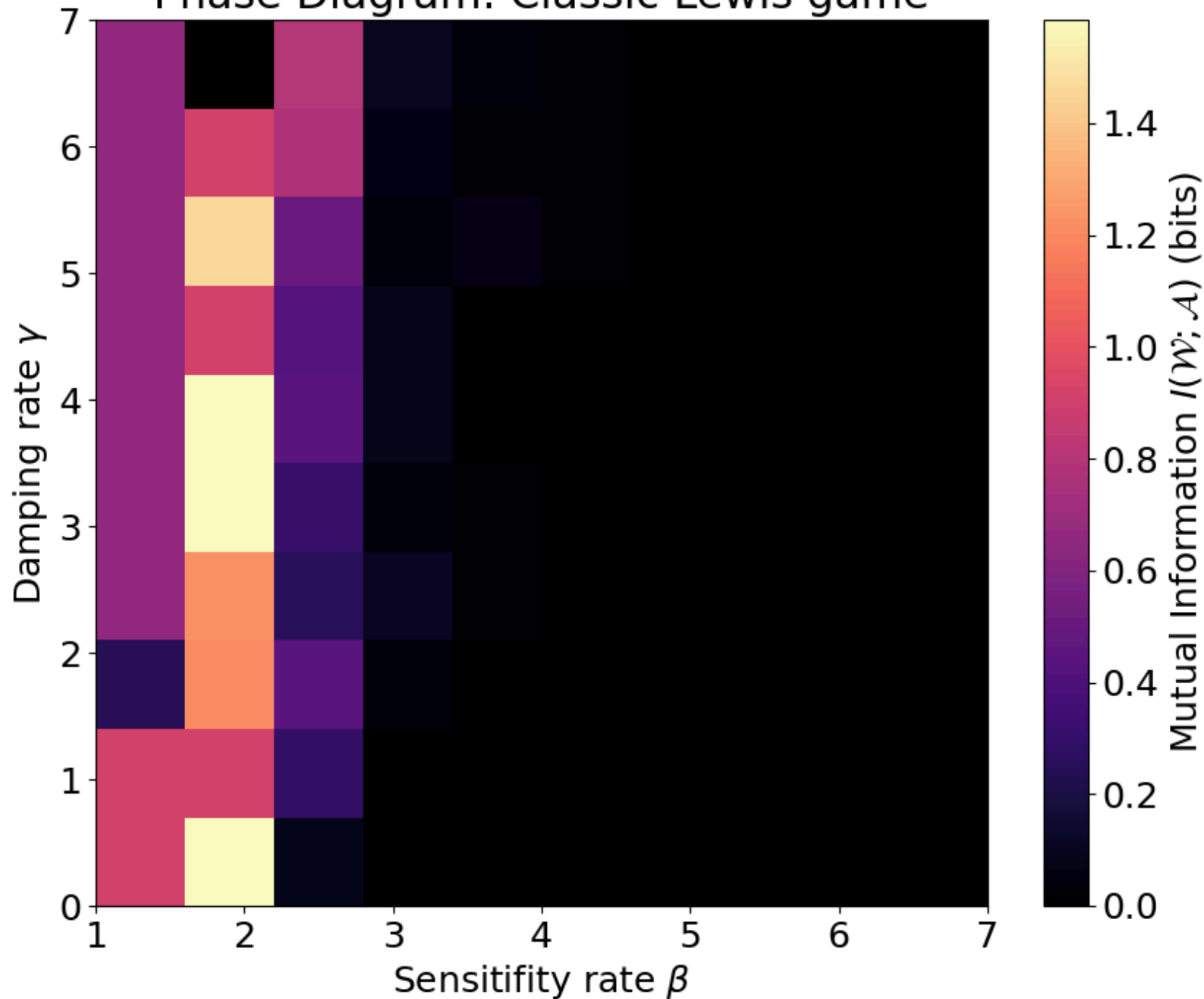
Phase Diagram: Classic Lewis game
