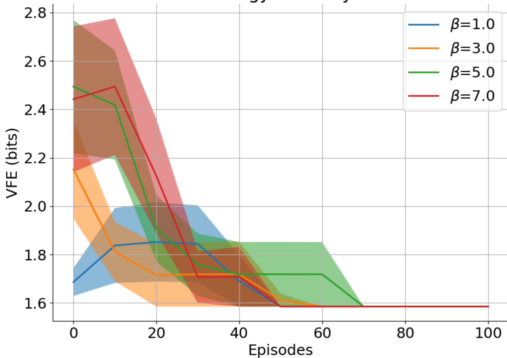
Free energy of the system
