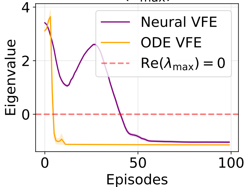
\text{Re}(\lambda_{\max})
