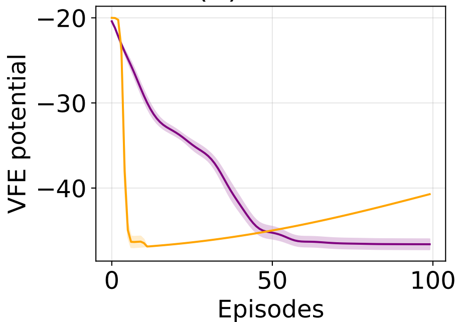
\mathcal{F}(\mathcal{Z}) descent
