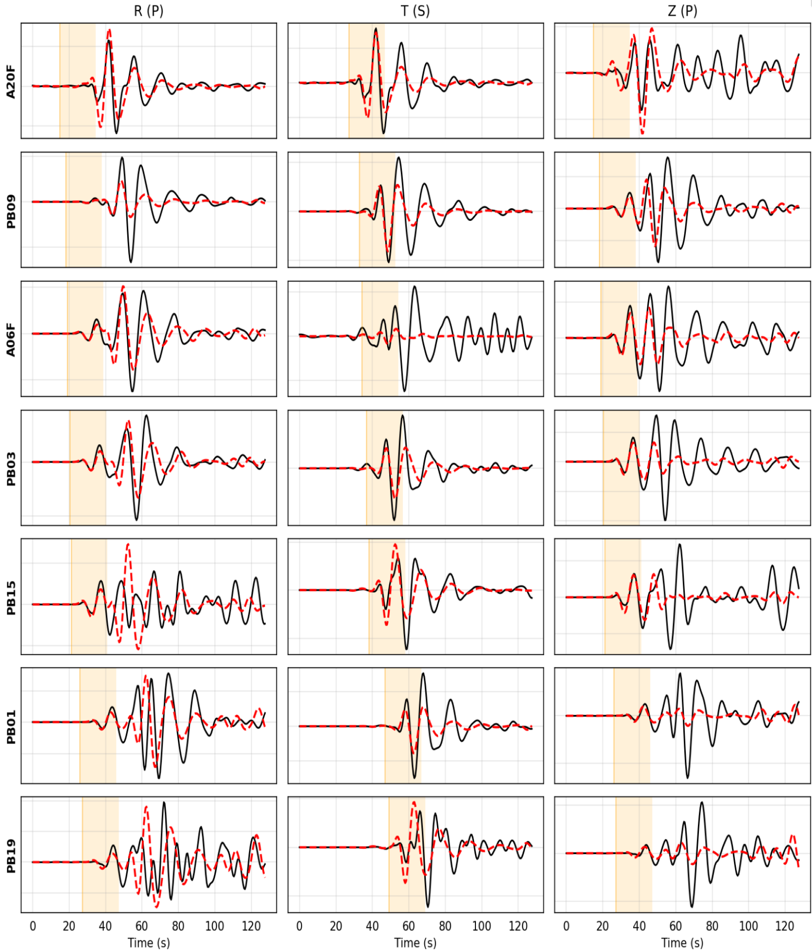
Posterior uncertainty — NA appraisal (1=0.334, N=4000)
