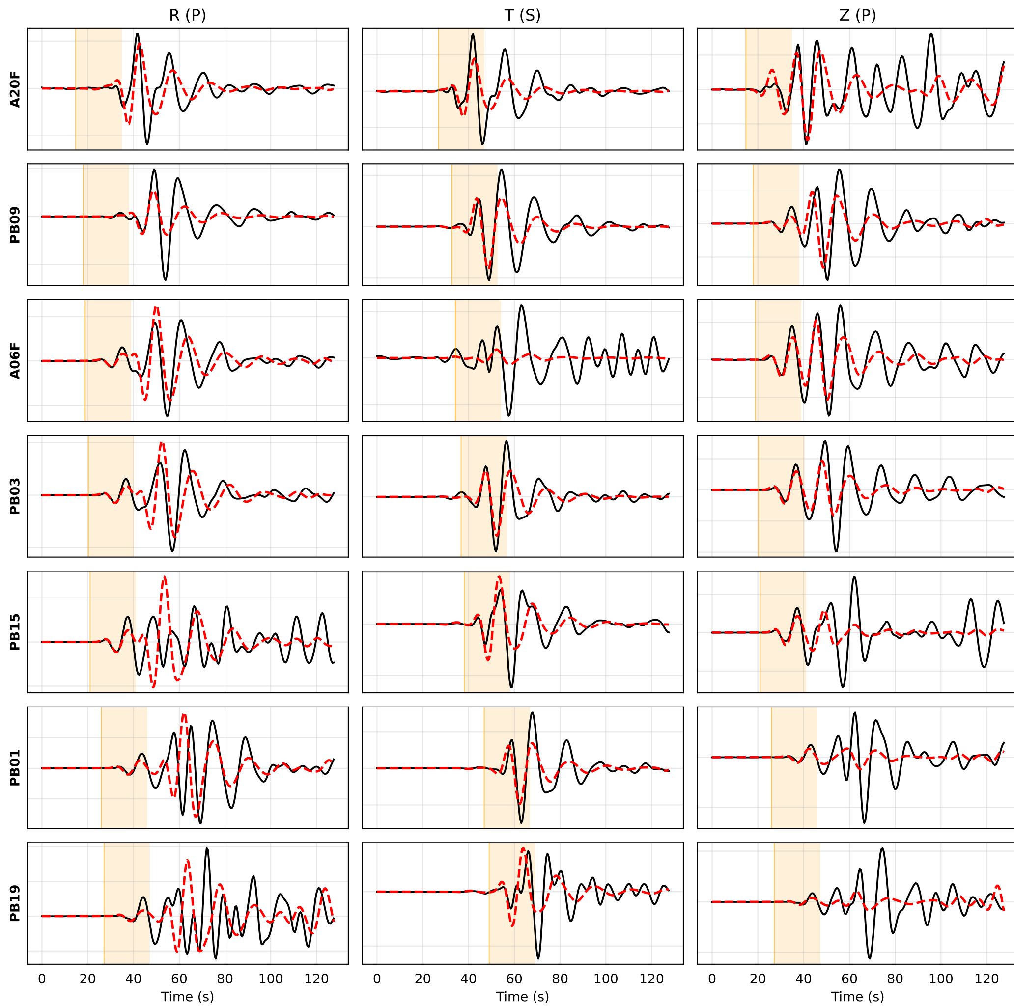
Waveform Fit (R/T/Z) · ventana 20s (P→R,Z ; S→T) (Misfit: 0.3717)
