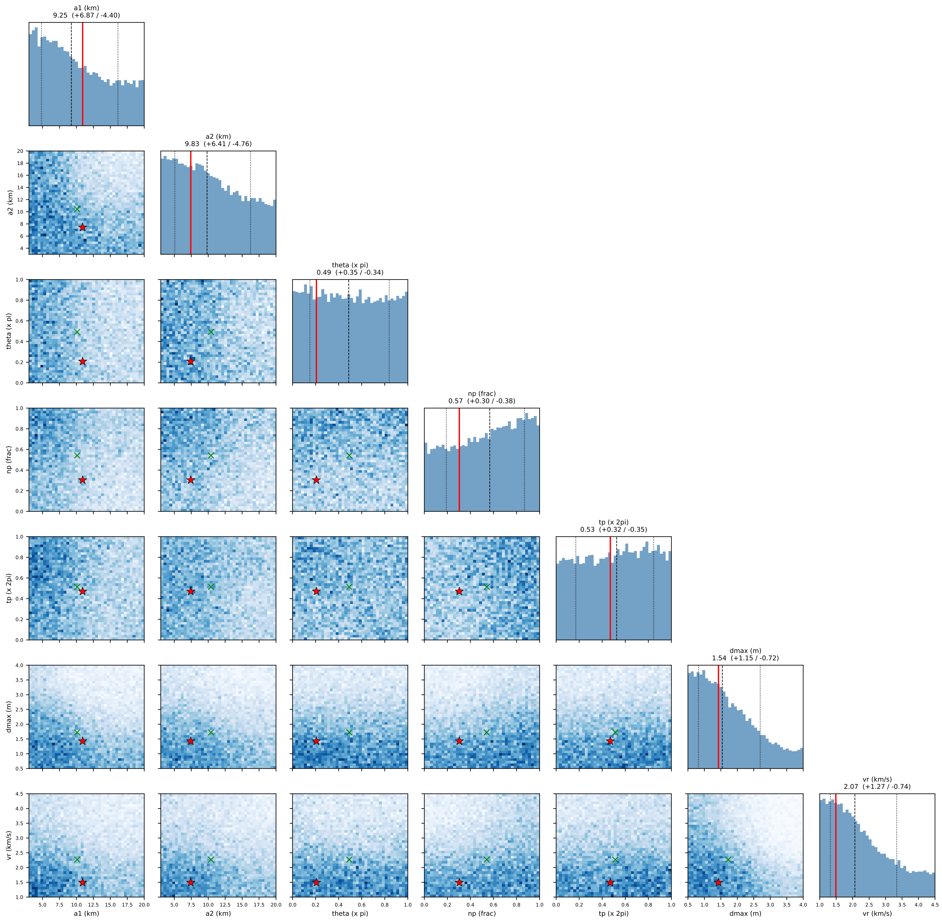
Posterior uncertainty — NA appraisal (T=0.743, N=20000)
