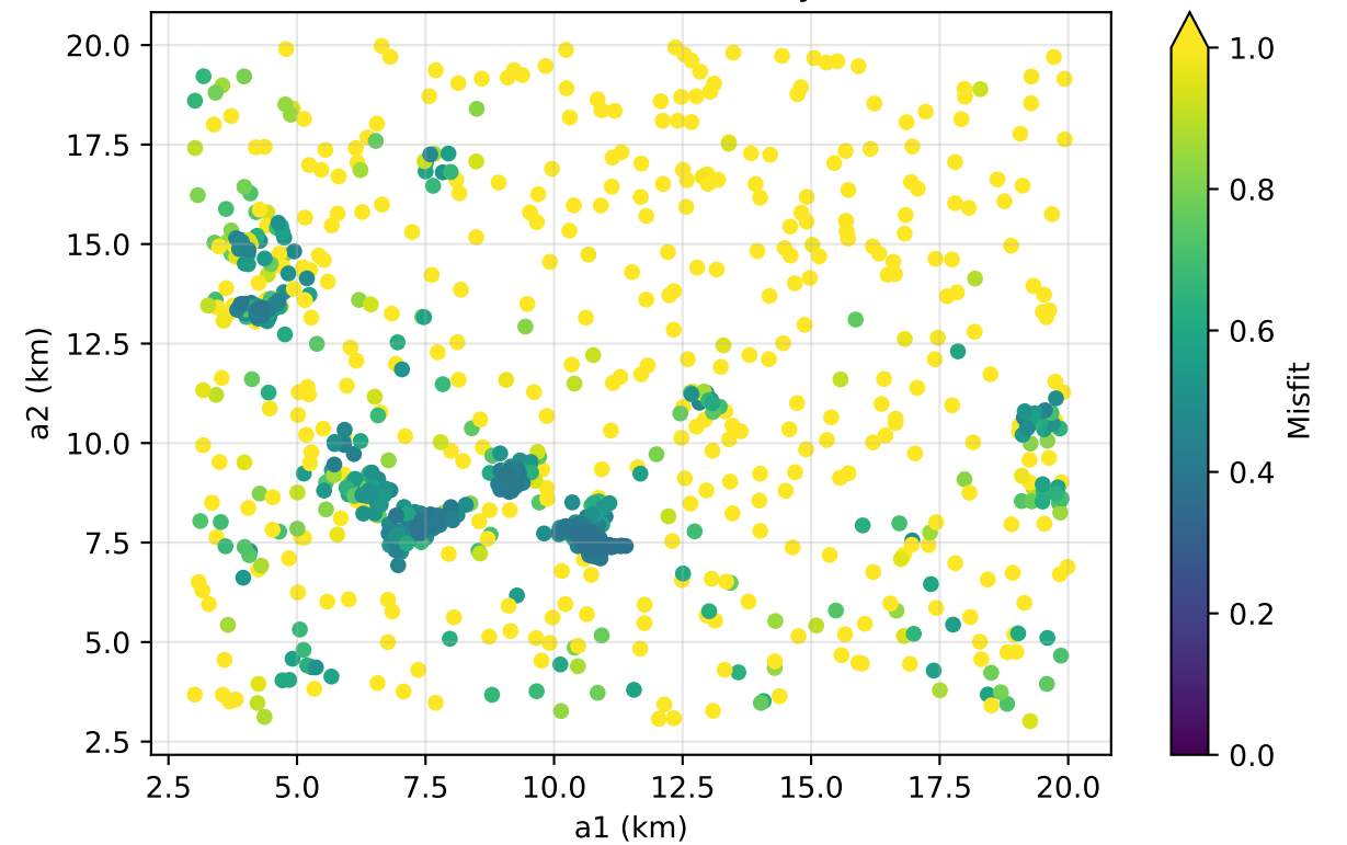
Parameter cloud colored by misfit
