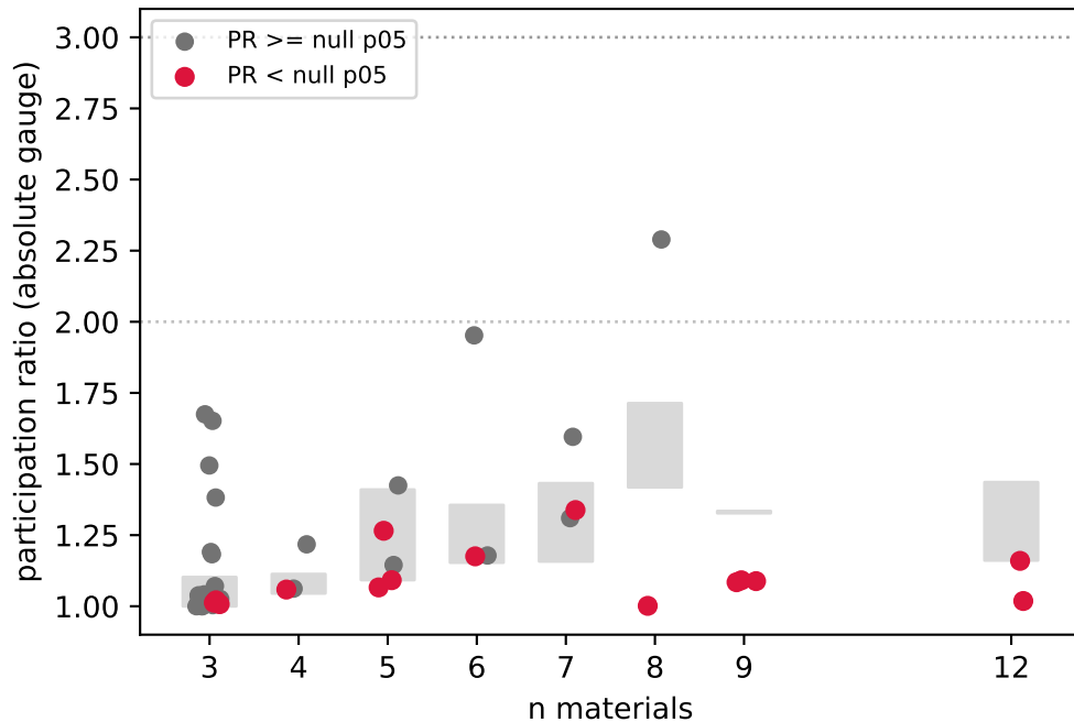
short_label lineage (42 groups)
