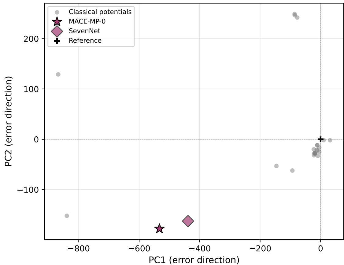
Mo (BCC)
