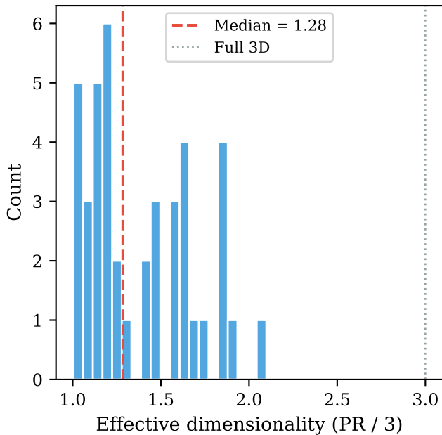
Distribution (N = 42)
