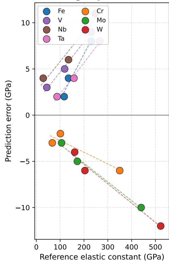
Within-group correlations
