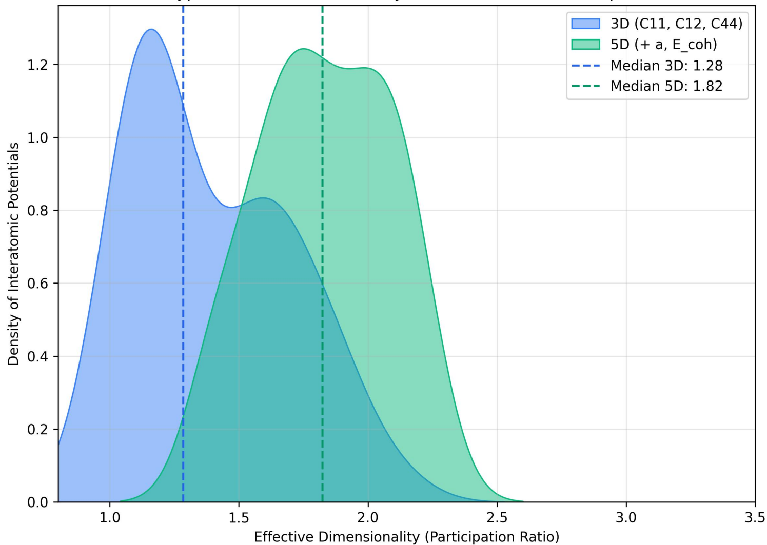
Hyper-Ribbon Dimensionality: 3D vs 5D Observation Space
