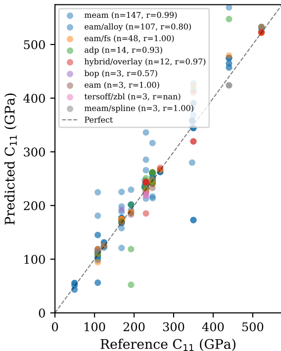
C_{11} : reference vs. predicted
