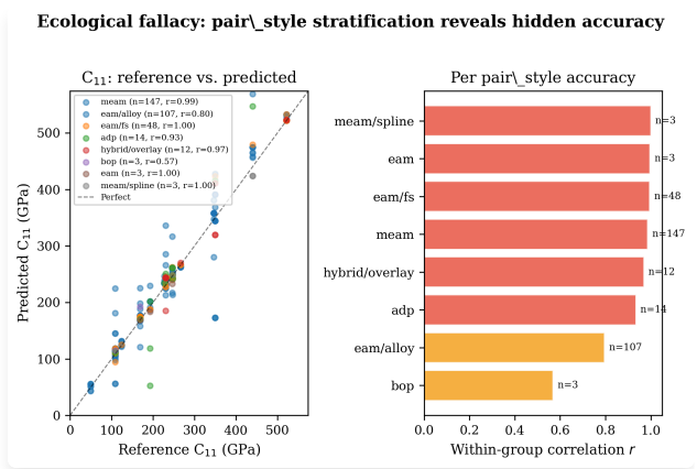
Pair_style stratification reveals ecological fallacy. Left: Reference vs. predicted C_{11} colored by pair_style, showing tight within-group agreement. Right: Per-pair_style correlations; pooled r = 0.82 understates within-group mean r = 0.95 .
