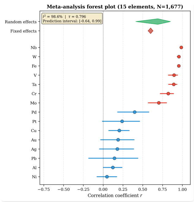
Meta-analysis forest plot. Individual elements colored by crystal structure (red = BCC, blue = FCC). Fixed- and random-effects summaries shown as diamonds. I^2 = 98.6\%
