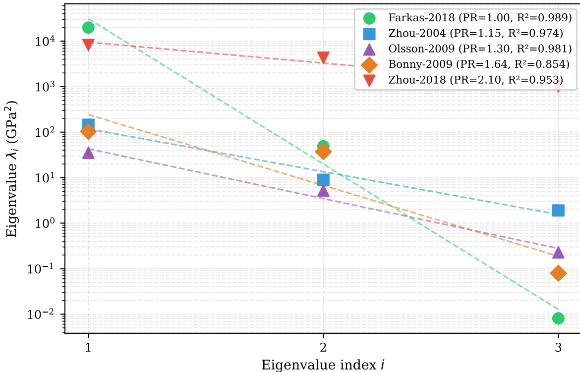
Elastic constant error eigenvalue spectra (real NIST/OpenKIM data)
