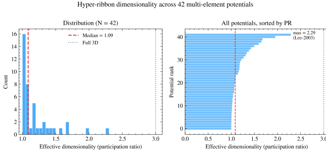
Figure 2: Distribution of effective dimensionality (participation ratio) across all multi-element potentials with \geq 3 materials. Median PR = 1.09 out of 3 (maximum 2.29); no potential approaches the full 3D space.
