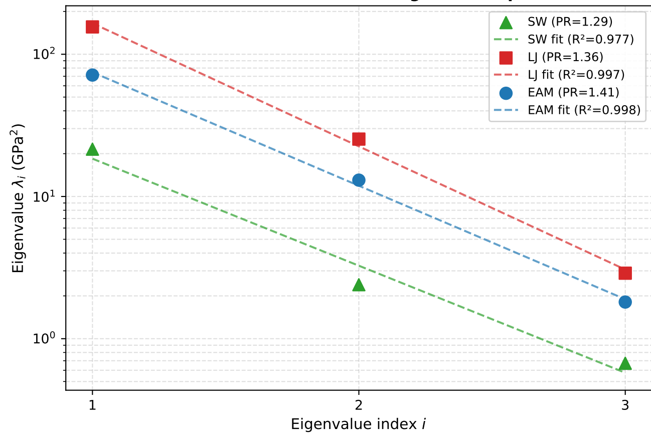
FCC elastic constant error eigenvalue spectra
