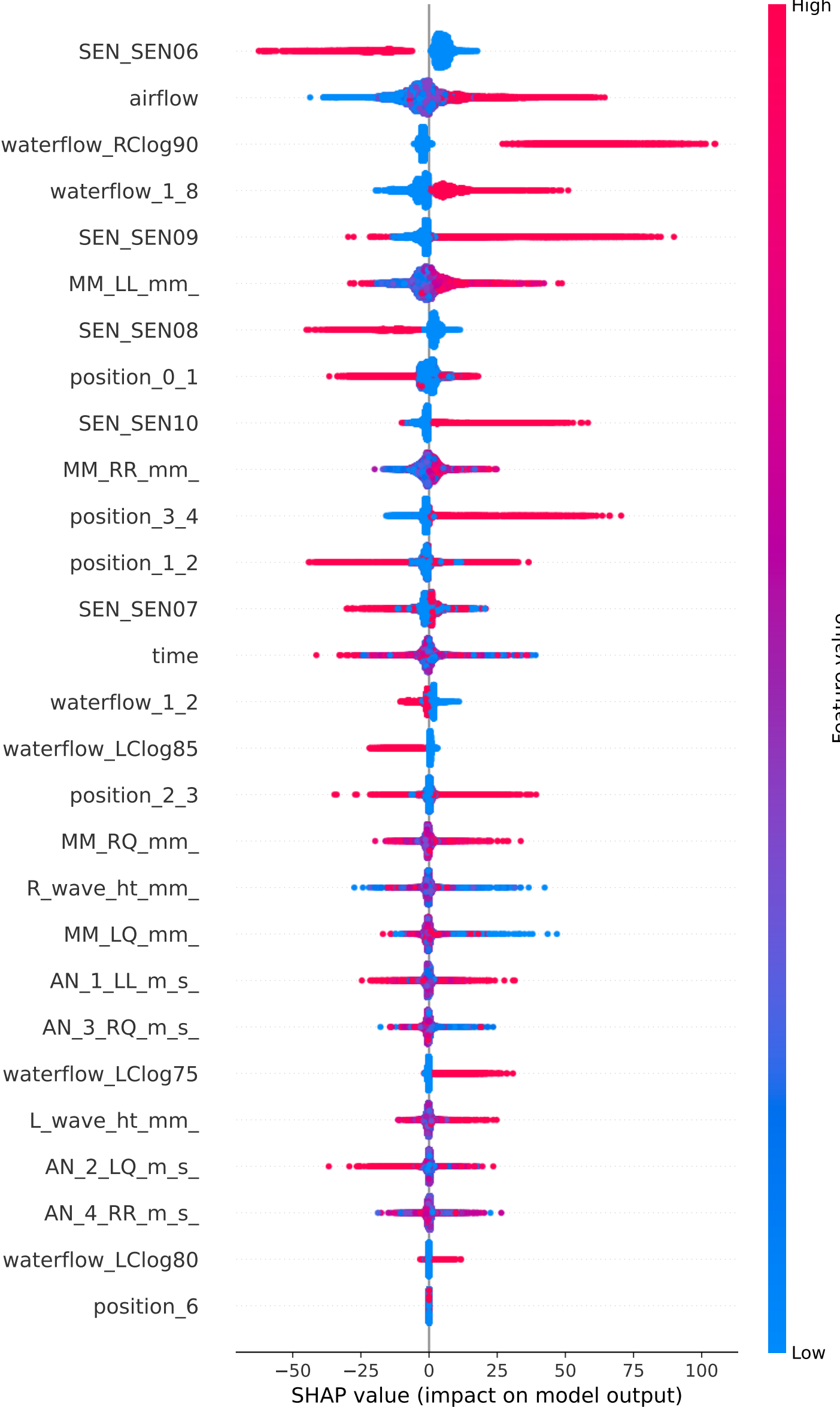
SHAP Beeswarm Plot for 20241206_Count_EX1_OneHot
