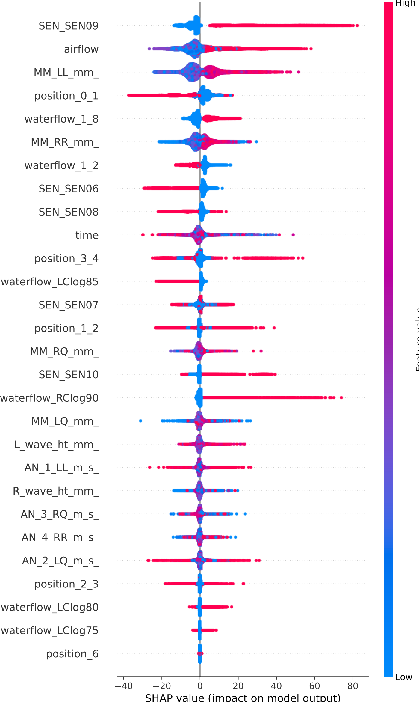
SHAP Beeswarm Plot for 20241206_Count_EX2_OneHot
