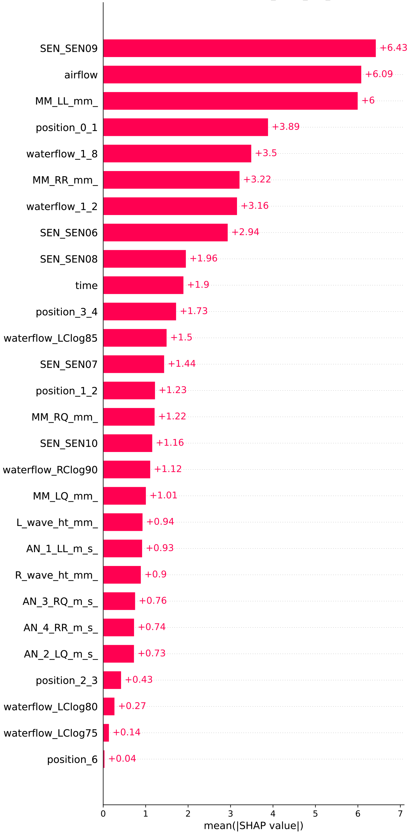
SHAP Bar Plot for 20241206_Count_EX2_OneHot
