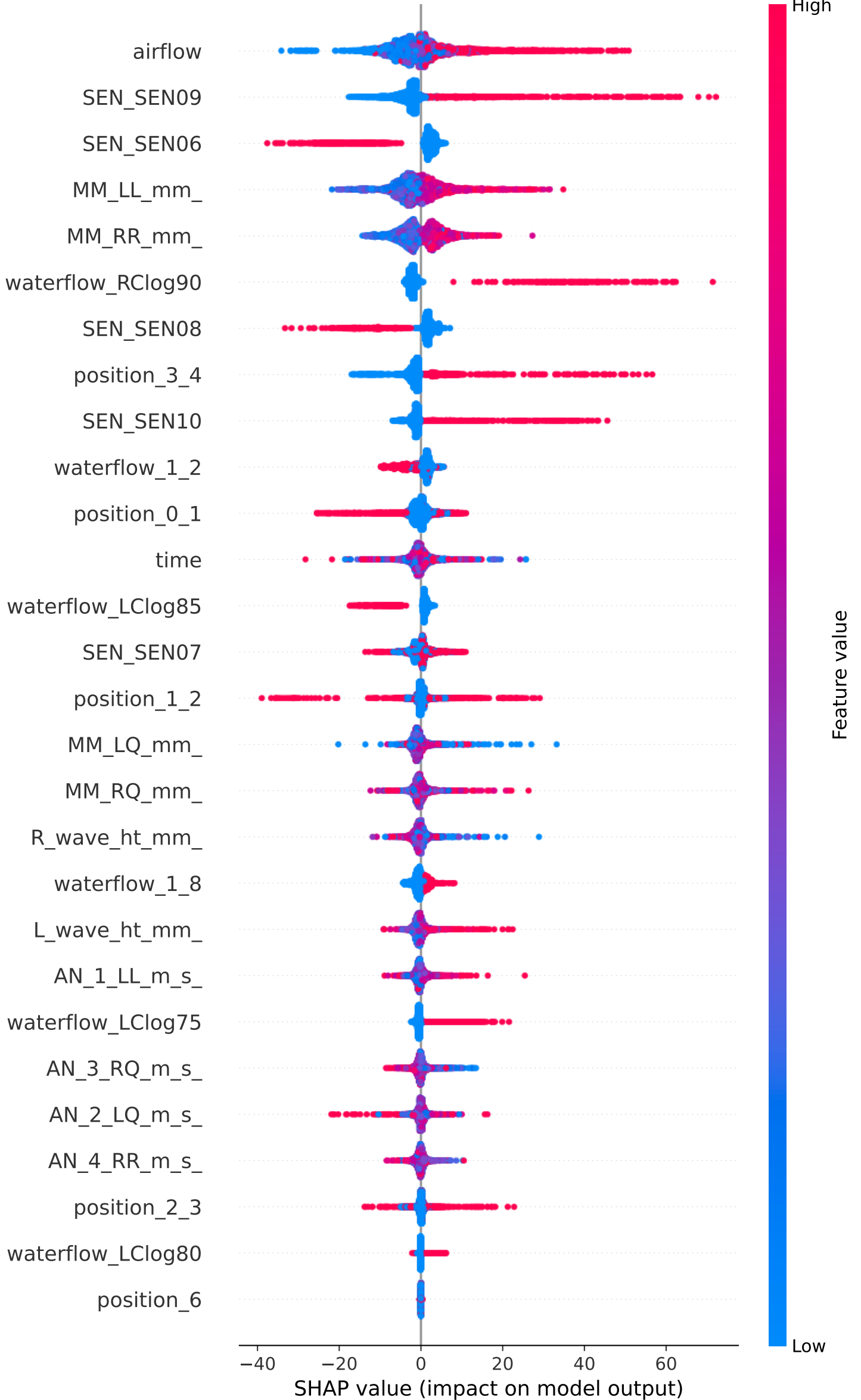
SHAP Beeswarm Plot for 20241008_all_features_Count_EX1_OneHot
