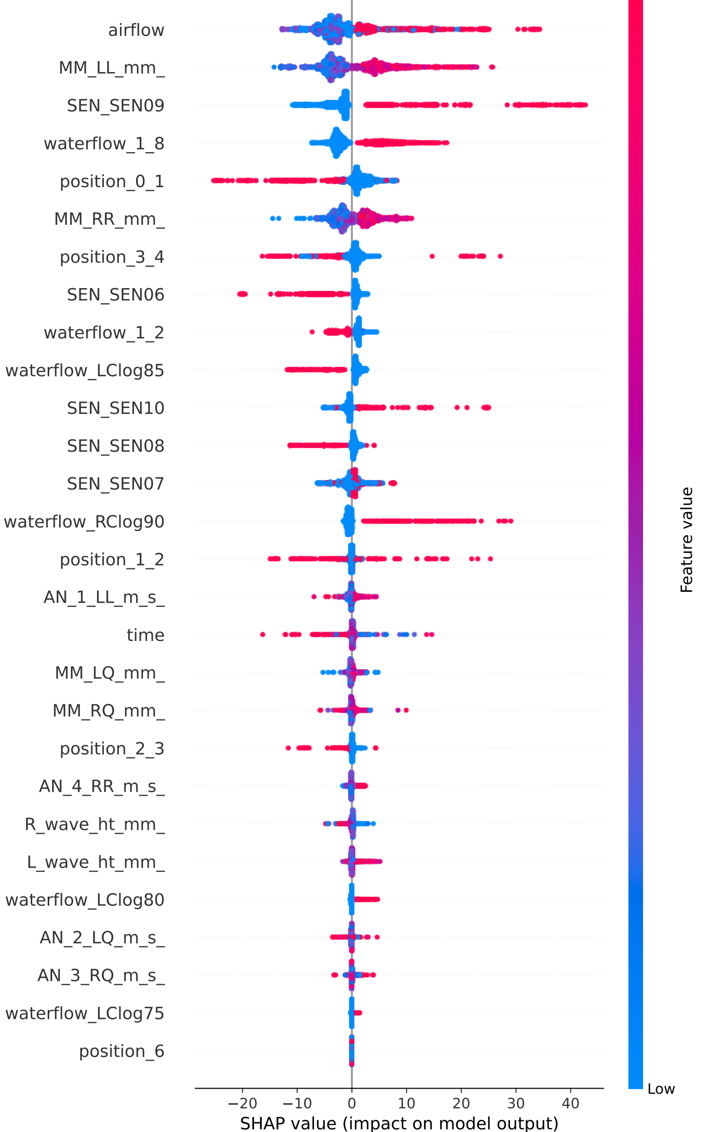
SHAP Beeswarm Plot for 20241008_all_features_Count_EX2_OneHot
