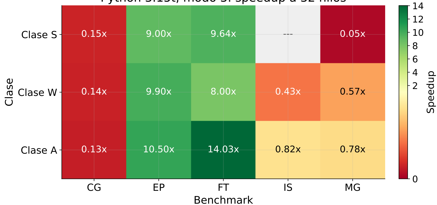
Python 3.15t, modo 3: speedup a 32 hilos
