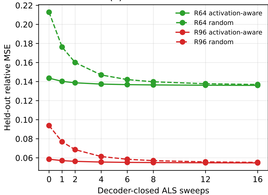
(a) Reconstruction
