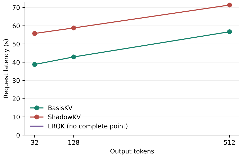
(b) 130048-token prompt, B1
