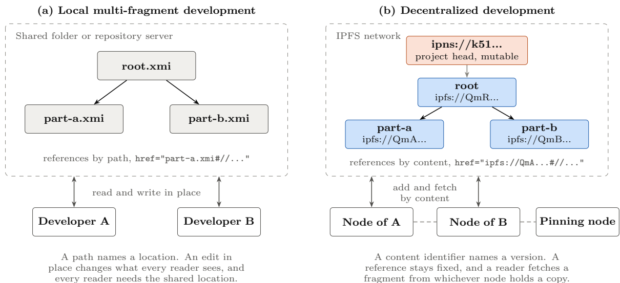
Figure 1: Development of a model that is split into fragments. (a) In a local setting, the fragments sit in one shared location, and each reference names a path. (b) In the decentralized setting of the study, each fragment is an immutable block on IPFS, each reference names a CID, and a mutable IPNS name marks the current version of the project.
