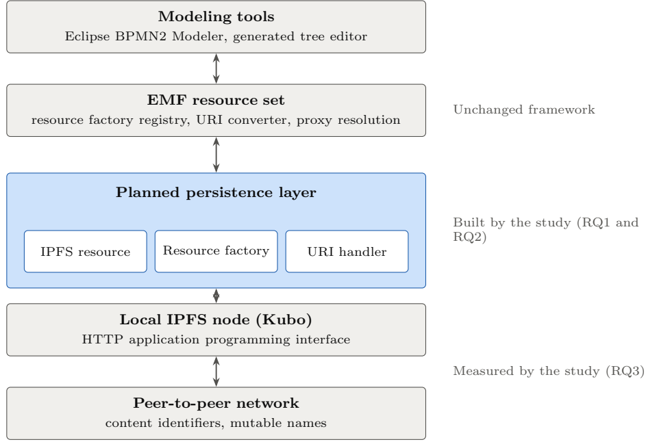
Figure 3: Planned place of the persistence layer. The framework above stays unchanged, the layer in the middle is the artifact of the study, and the node below gives the storage.
