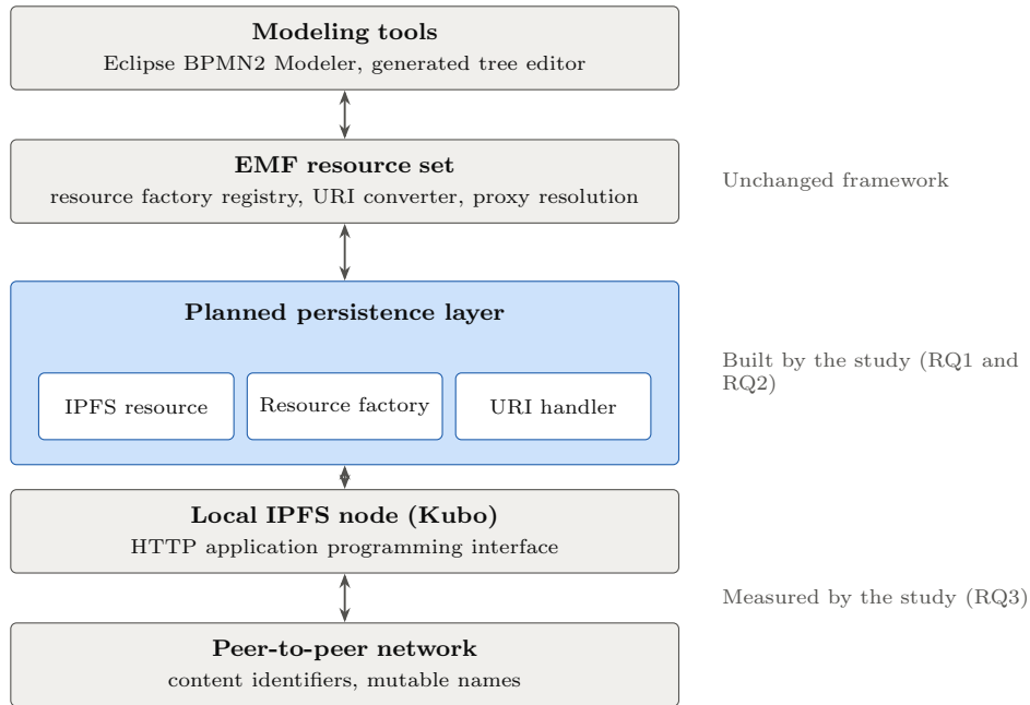
Figure 2: Planned place of the persistence layer. The framework above stays unchanged, the layer in the middle is the artifact of the study, and the node below gives the storage.
