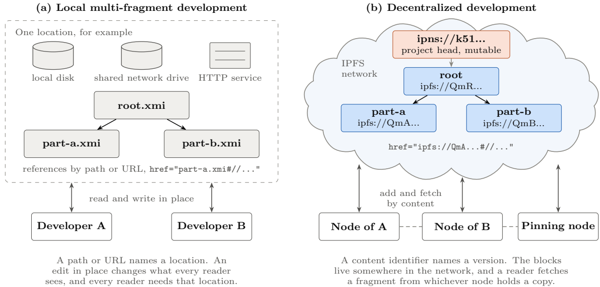
Figure 1: Development of a model that is split into fragments. (a) In a local setting, the fragments sit in one shared location, and each reference names a path. (b) In the decentralized setting of the study, each fragment is an immutable block on IPFS, each reference names a CID, and a mutable IPNS name marks the current version of the project.
