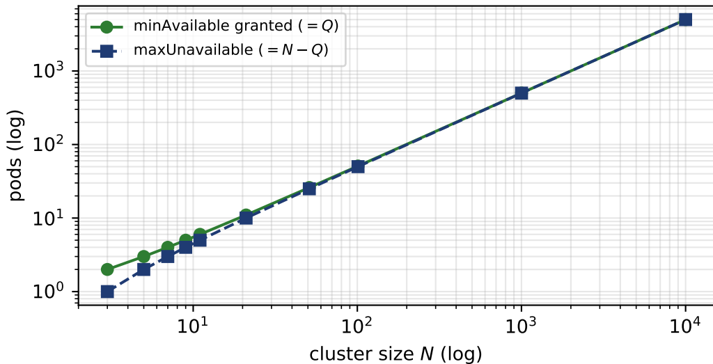
Budget tracks majority quorum as N scales
