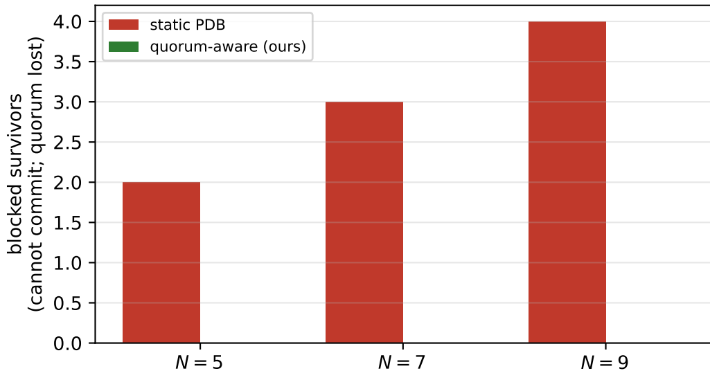
Quorum-gated workload stalled during rollout (RQ8)
