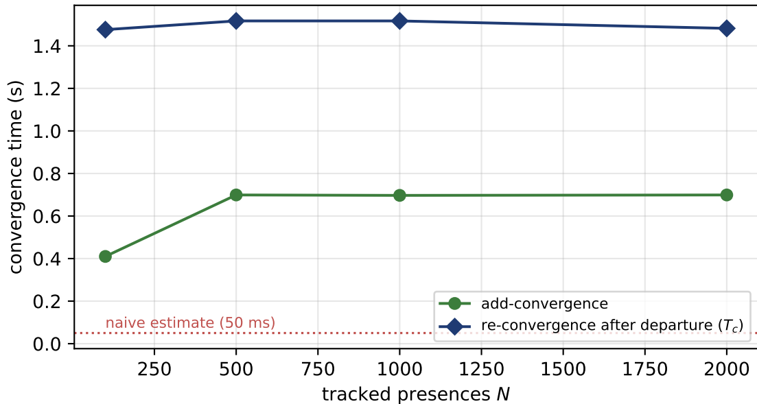
Phoenix.Presence convergence (realistic workload)
