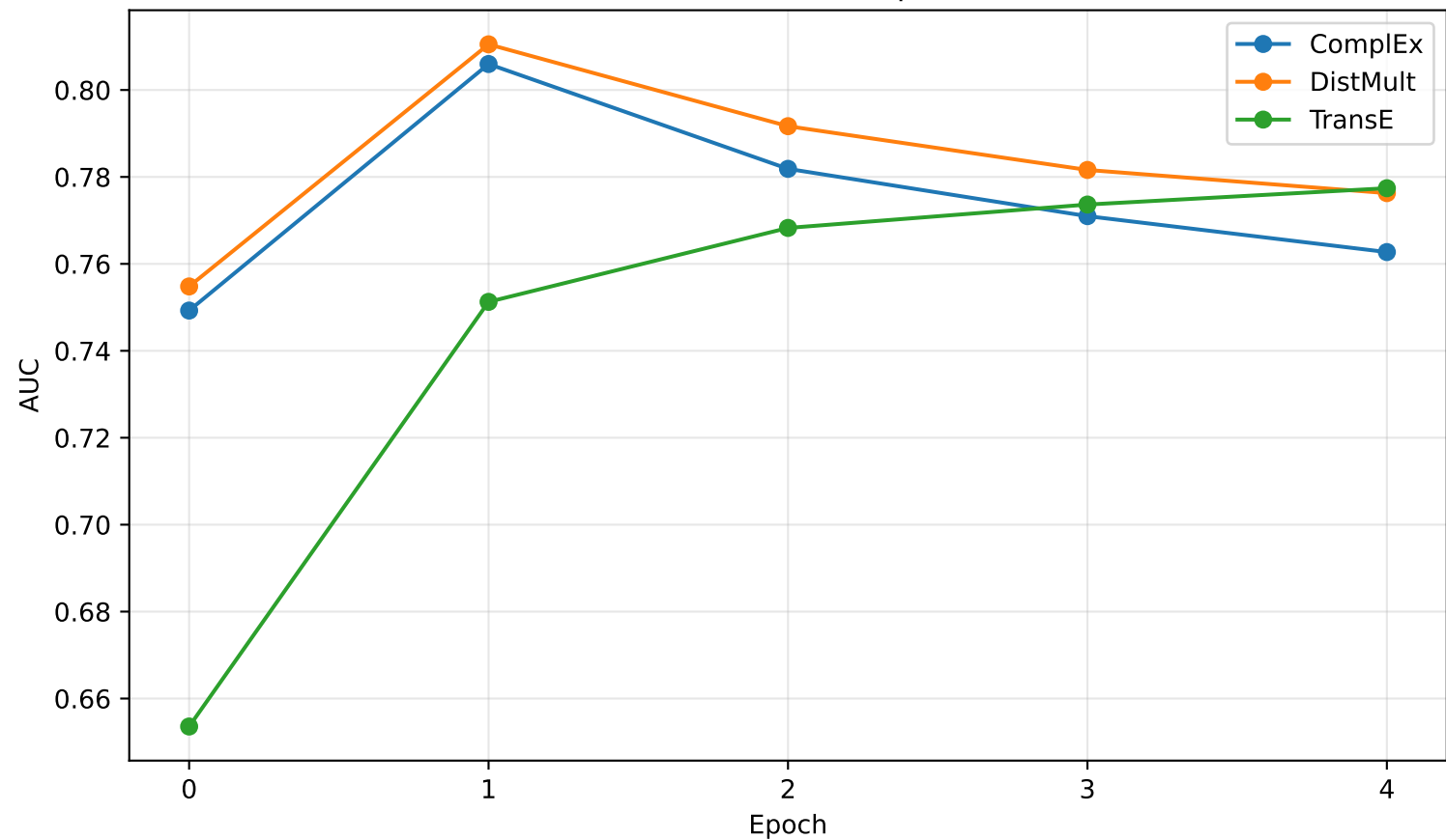
YAGO: AUC across epochs
