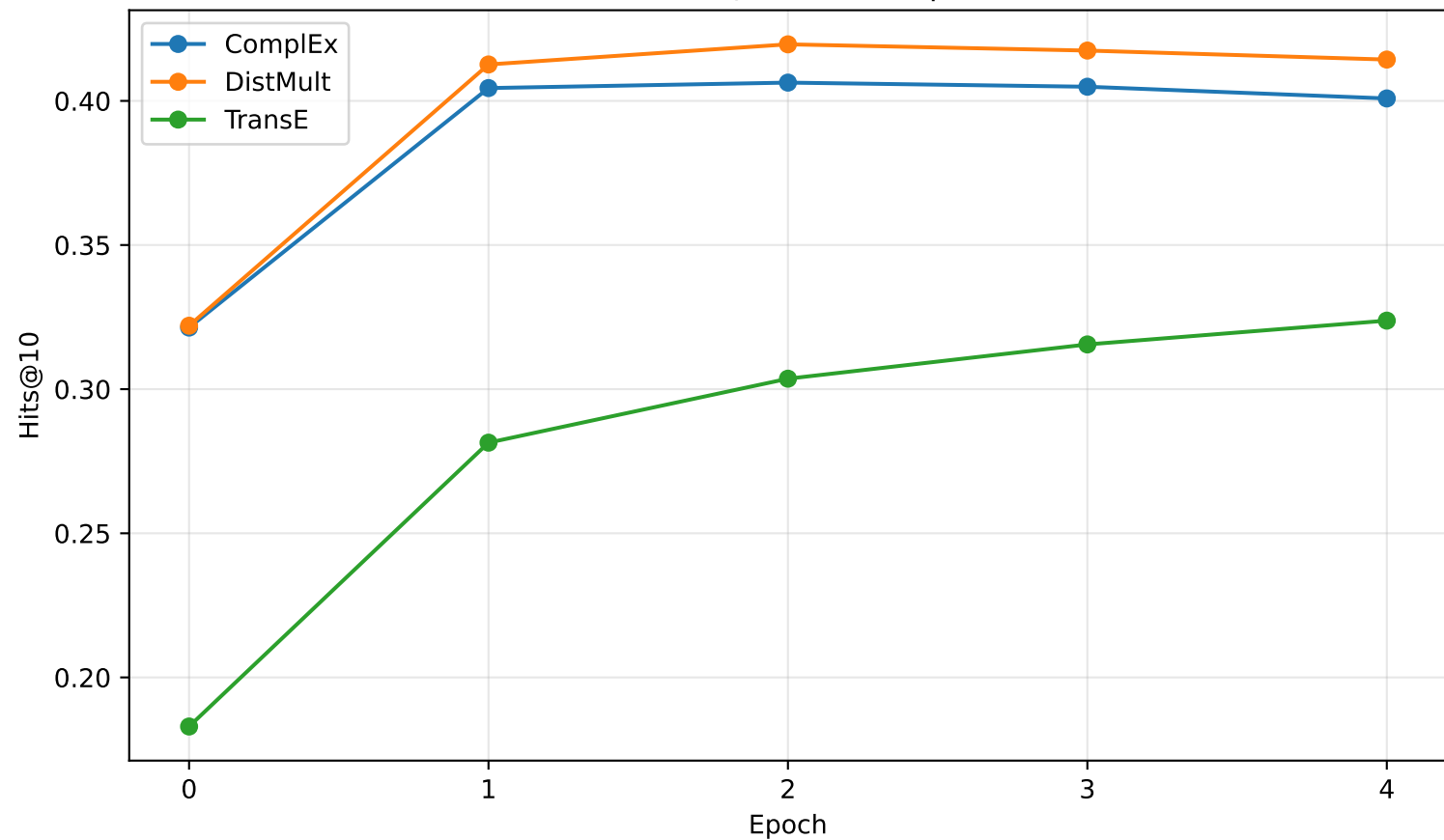
YAGO: Hits@10 across epochs
