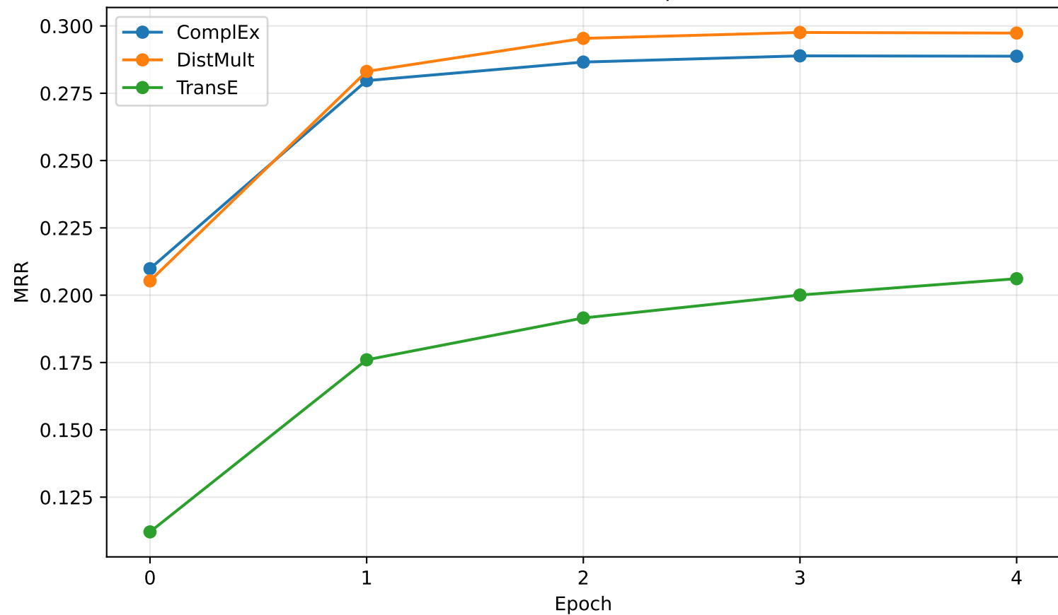
YAGO: MRR across epochs
