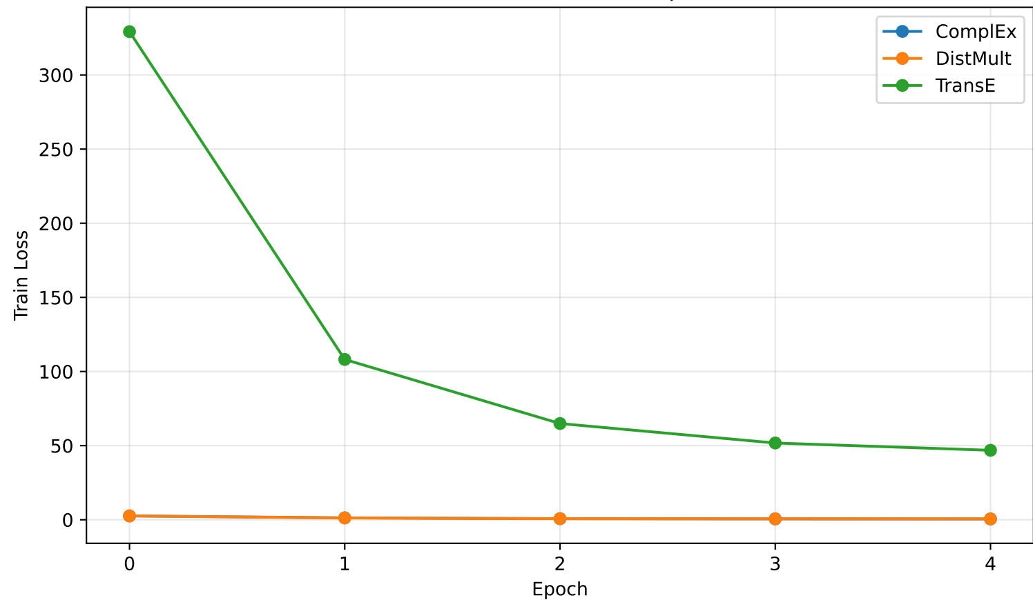
YAGO: Train Loss across epochs
