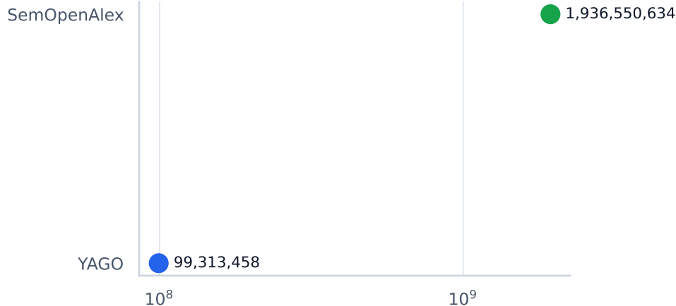
Structural triples
