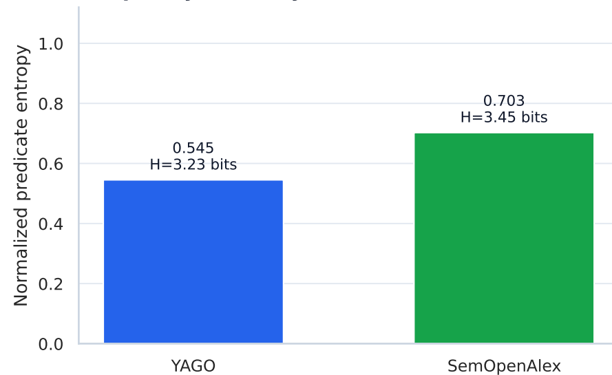
Frequency diversity
