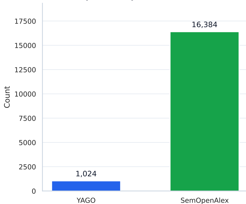
Possible partition pairs
