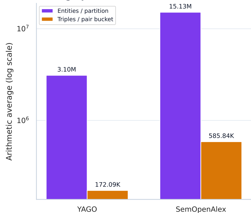
Average partition scale
