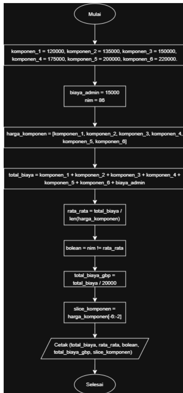
Gambar 1.1 Flowchart
