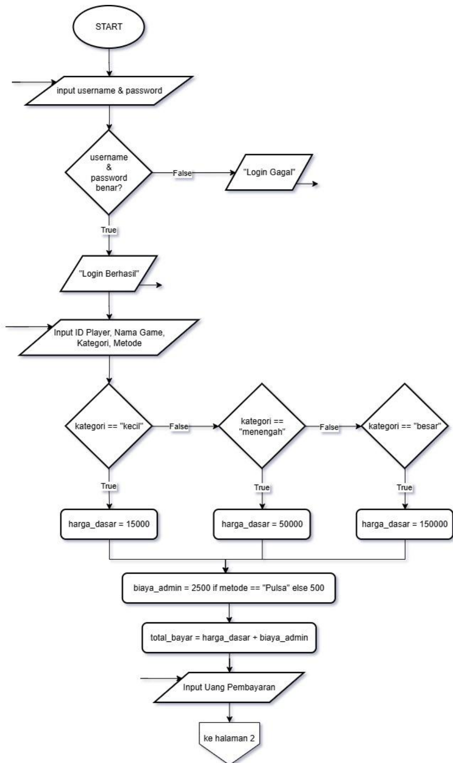
Gambar 1.1 Flowchart Halaman 1
