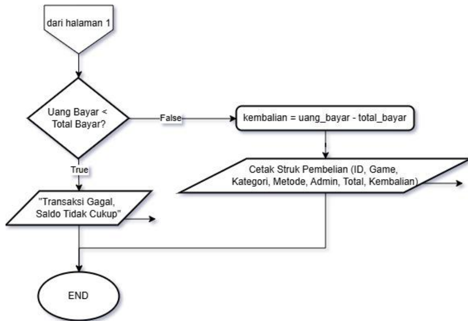
Gambar 1.2 Flowchart Halaman 2
