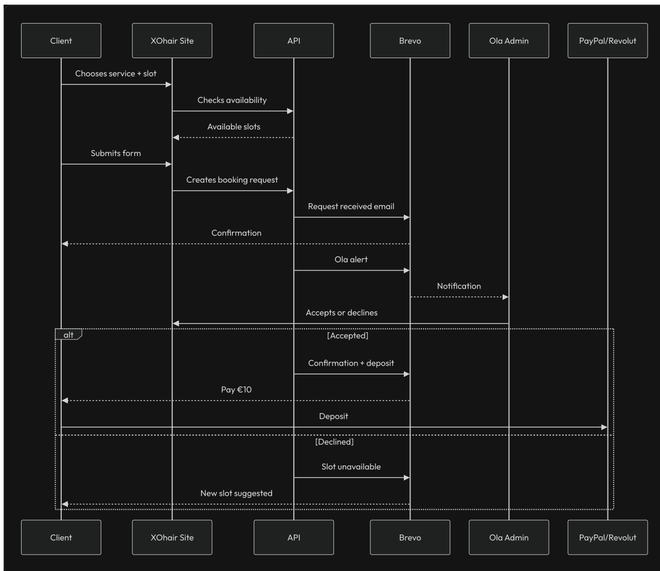
Figure 2 — Client journey from booking to confirmation
