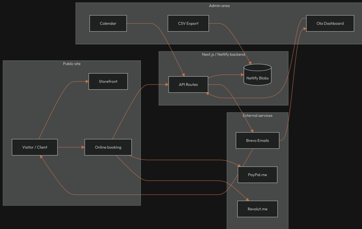
Figure 1 — Functional architecture of the XOhair Melun website
