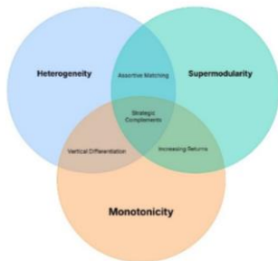
Fig. 2: Optimal Matching with Peer Effects
