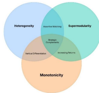
Fig. 2: Optimal Matching with Peer Effects
