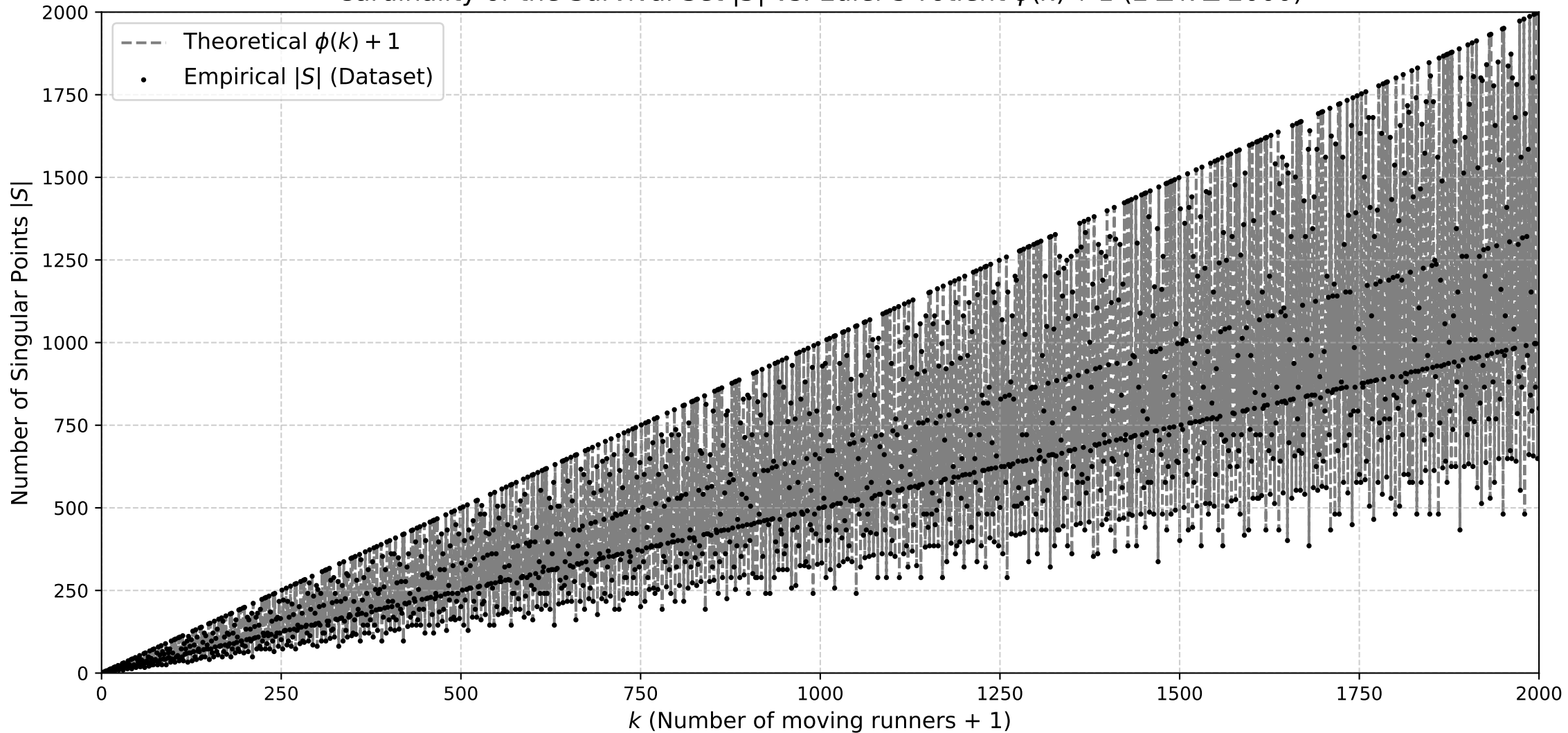
Cardinality of the Survival Set |S| vs. Euler's Totient \phi(k) + 1 ( 2 \leq k \leq 2000 )
