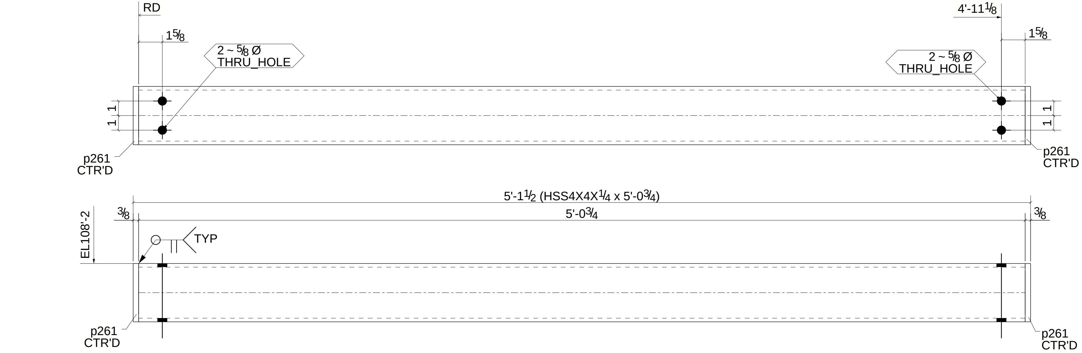
2 - BEAMS - 607B1
