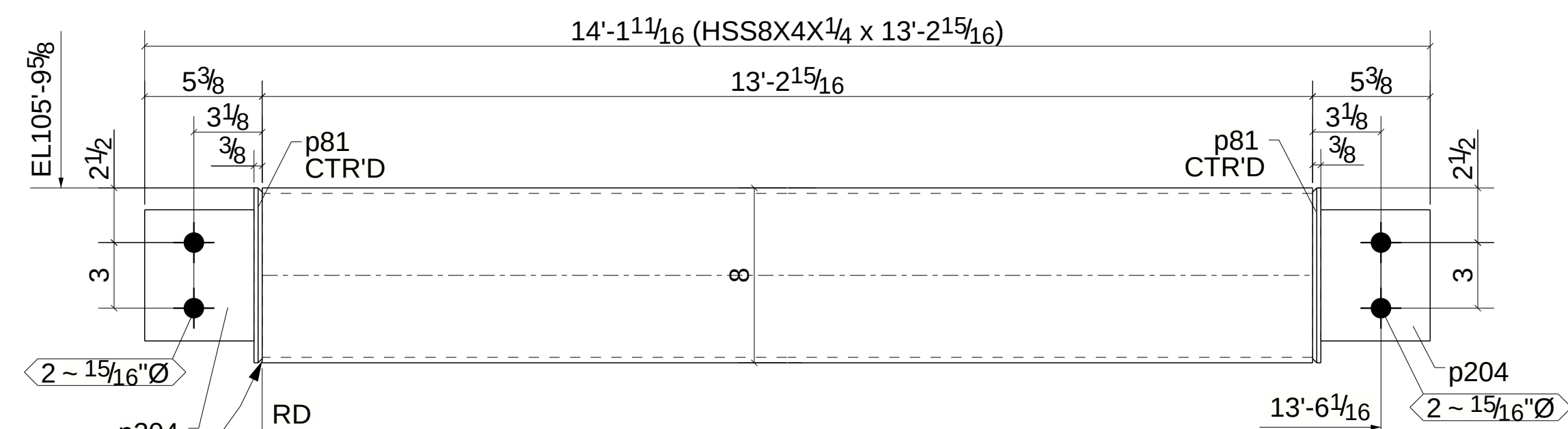
ONE - BEAM - 612B1
