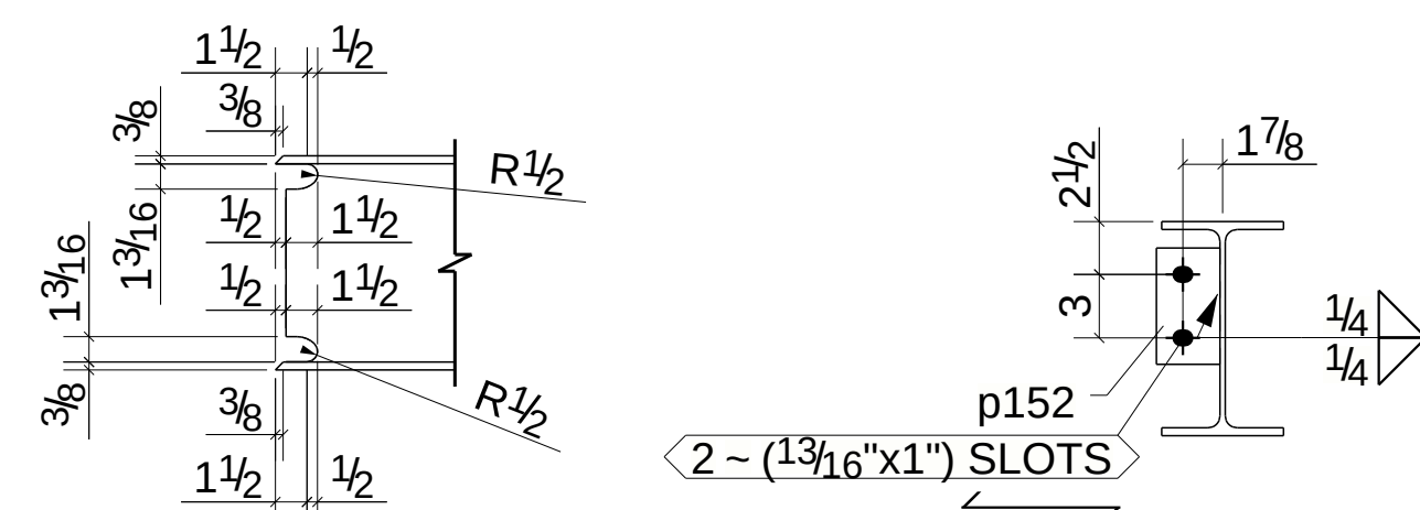
DETAIL 1
