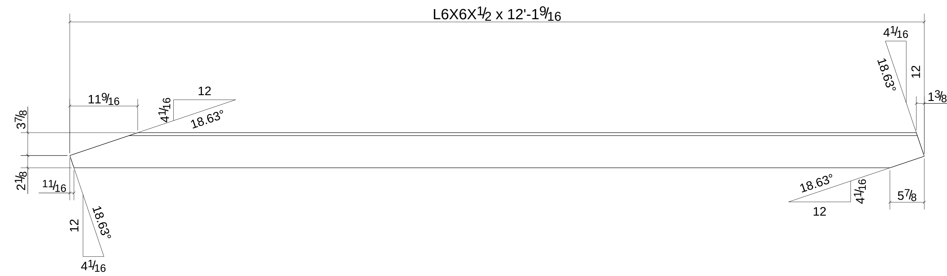
ONE - HORIZONTAL BRACE - 640HB4
