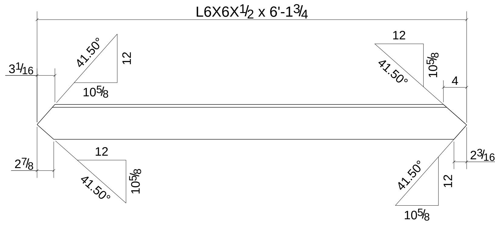
2 - HORIZONTAL BRACES - 640HB1
