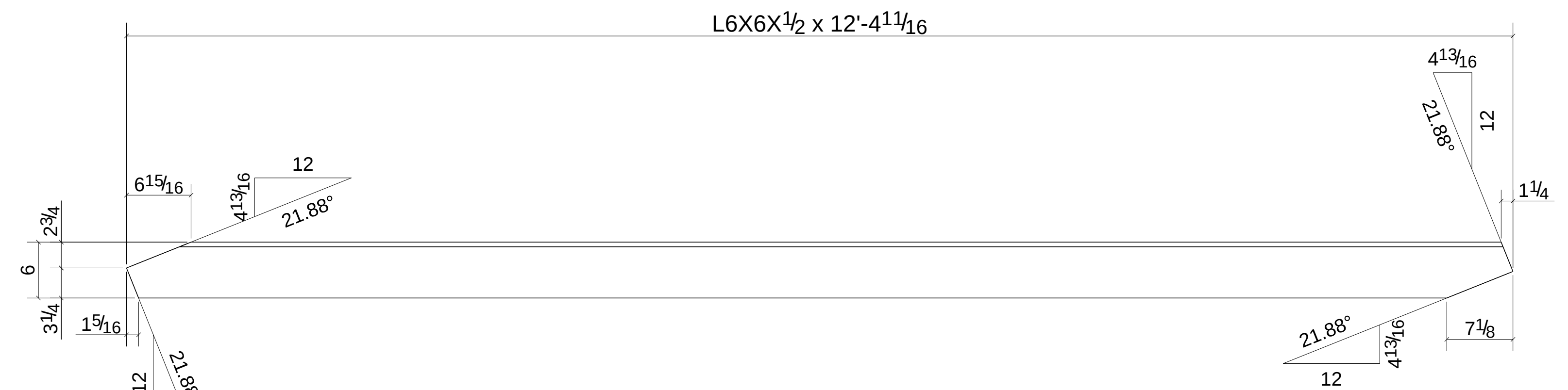
ONE - HORIZONTAL BRACE - 640HB5
