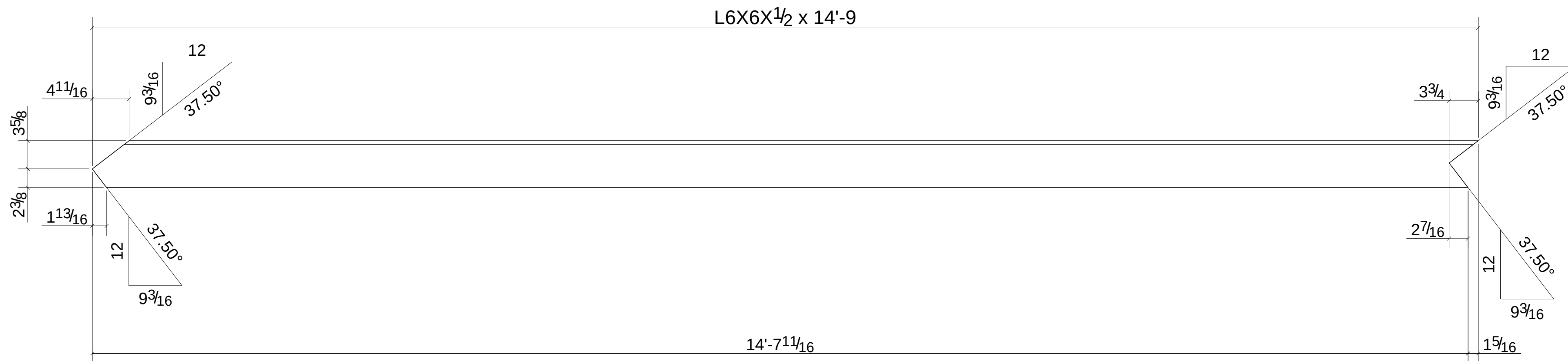
ONE - HORIZONTAL BRACE - 640HB3
