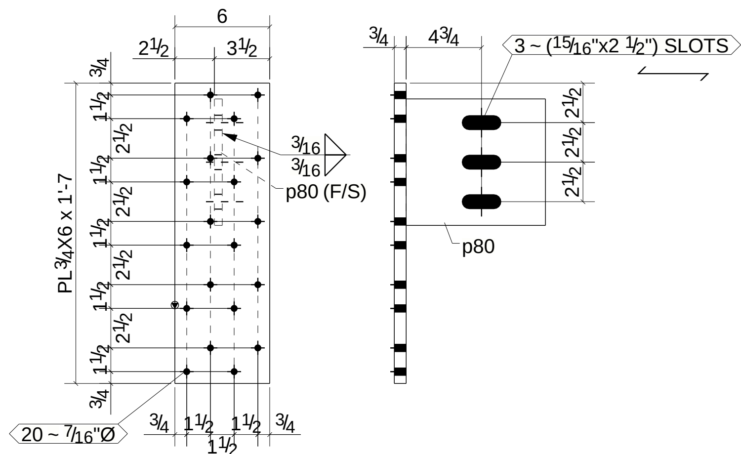
ONE - END PLATE - 643PL4
