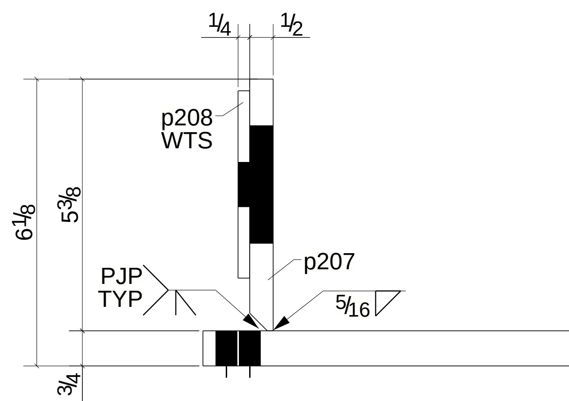
2 - END PLATES - 643PL3
