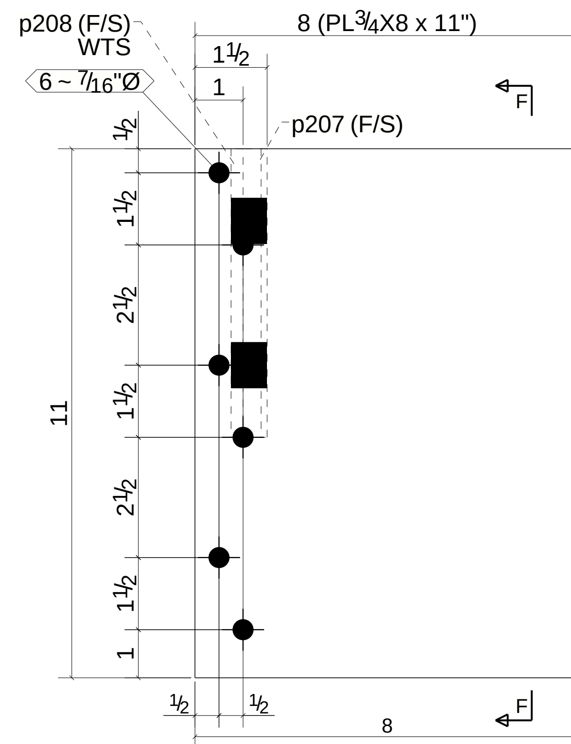
ONE - BASE PLATE - 643PL6
