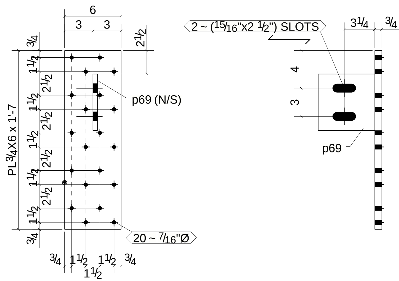
ONE - END PLATE - 643PL1
