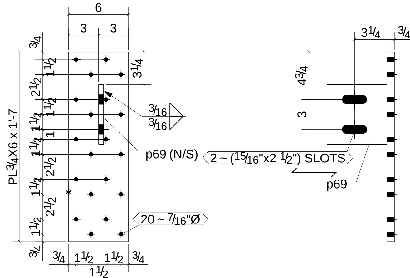
ONE - END PLATE - 643PL2
