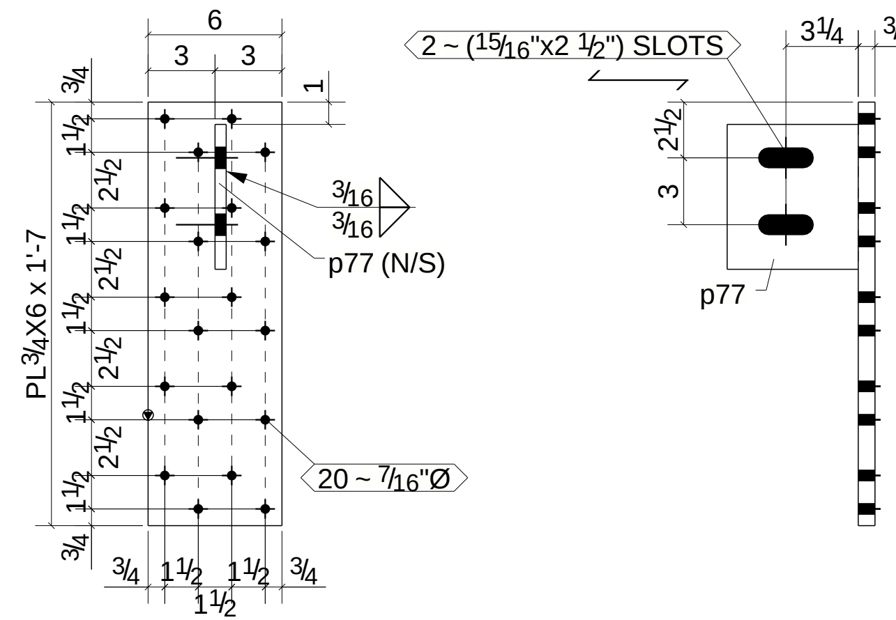
2 - END PLATES - 643PL3
