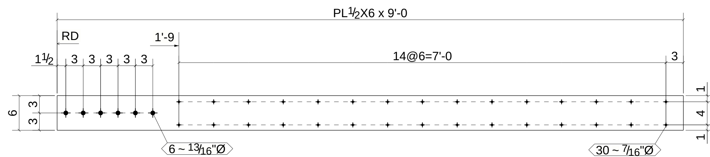
ONE - DRAG PLATE - 645PL2
