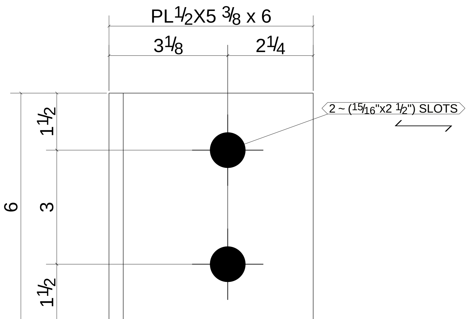
3 - SIDE PLATES - 645PL1
