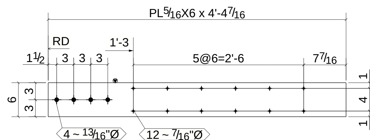
ONE - DRAG PLATE - 645PL4
