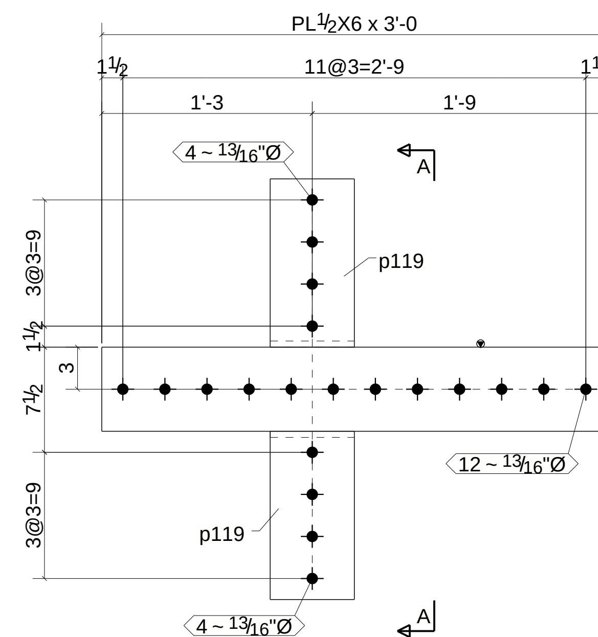
ONE - SPLICE PLATE - 645PL6
